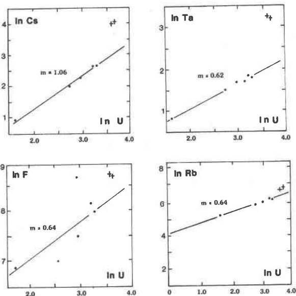
Fig. 4. Logarithmic variation diagrams for topaz rhyolites from the Thomas Range (o) and Spor Mountain (+). The lines represent least-squares fits to the data from the Thomas Range. The bulk partition coefficient ( \bar{D} ) for each element is derived from the equation \bar{D} = 1 - m , where m is the slope of the line (see text).
